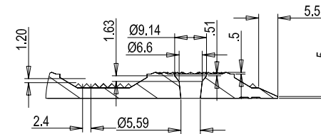
DETAIL D SCALE 4
