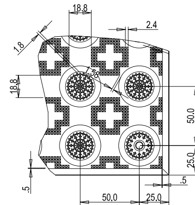
DETAIL E SCALE 2
